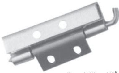
Concealed Hinge 180°
